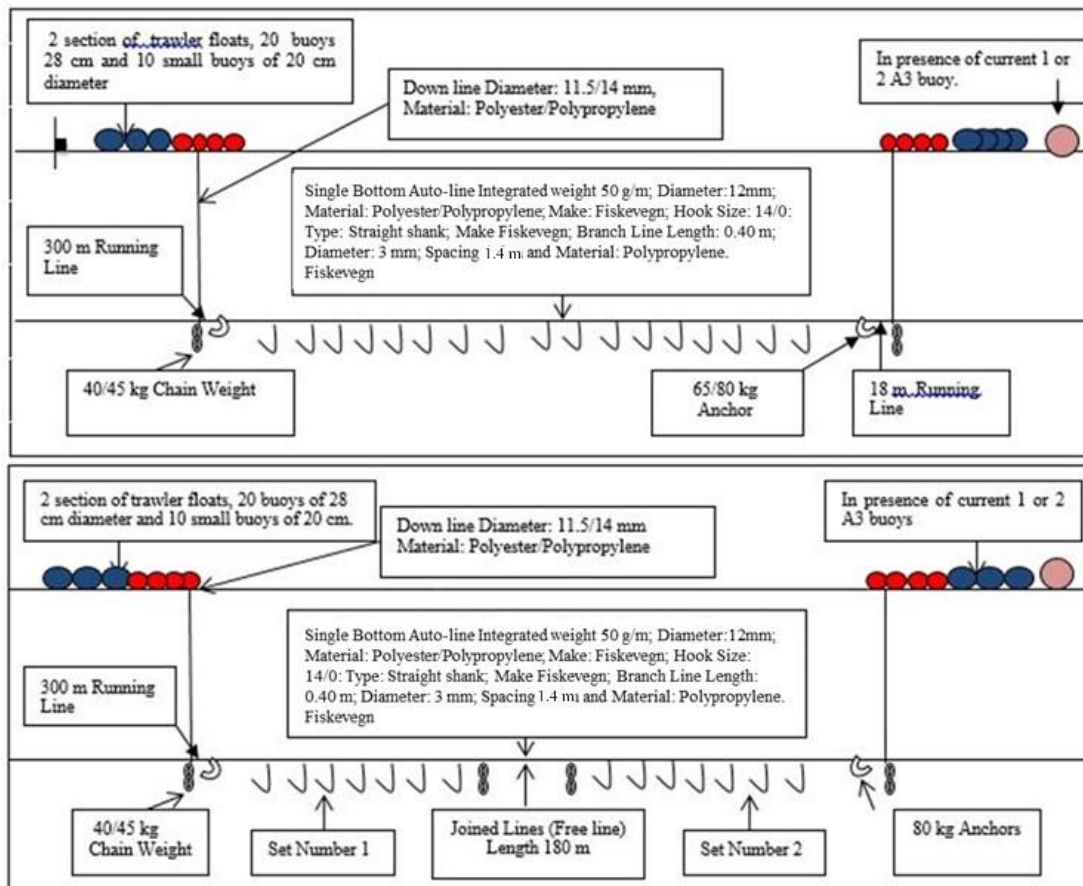
Figure 1 The e gear configurations for Argos Froyanes
