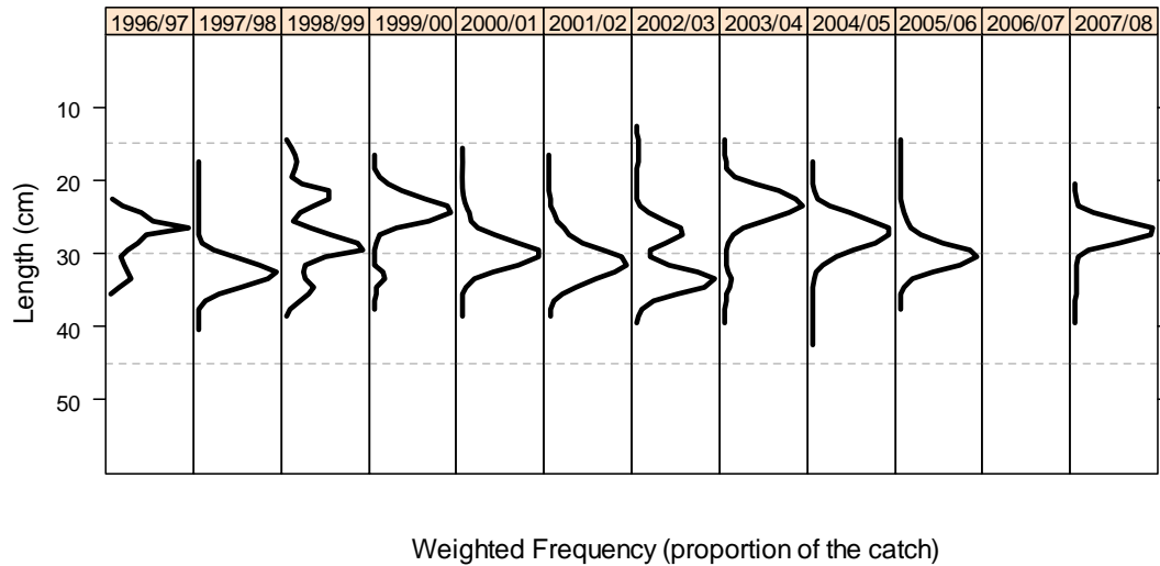
Figure 1: Catch-weighted length frequencies for Champsocephalus gunnari in Division 58.5.2 (source: observer, fine-scale and STATLANT data). The plots include data from both the commercial fishery and research trawl surveys.
