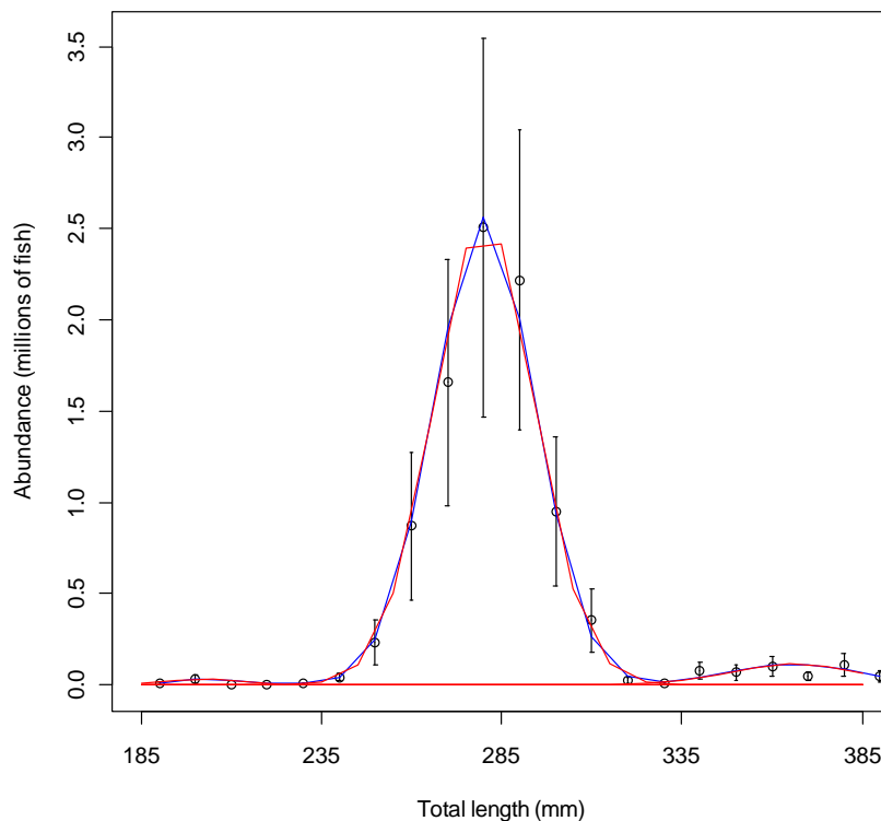
Figure 3: Size distribution of Champsocephalus gunnari from the 2008 random stratified trawl survey in Division 58.5.2 with standard errors. Cohorts were present in ages 1, 2, 3 and 4. The plot is dominated by age-2+ fish.
