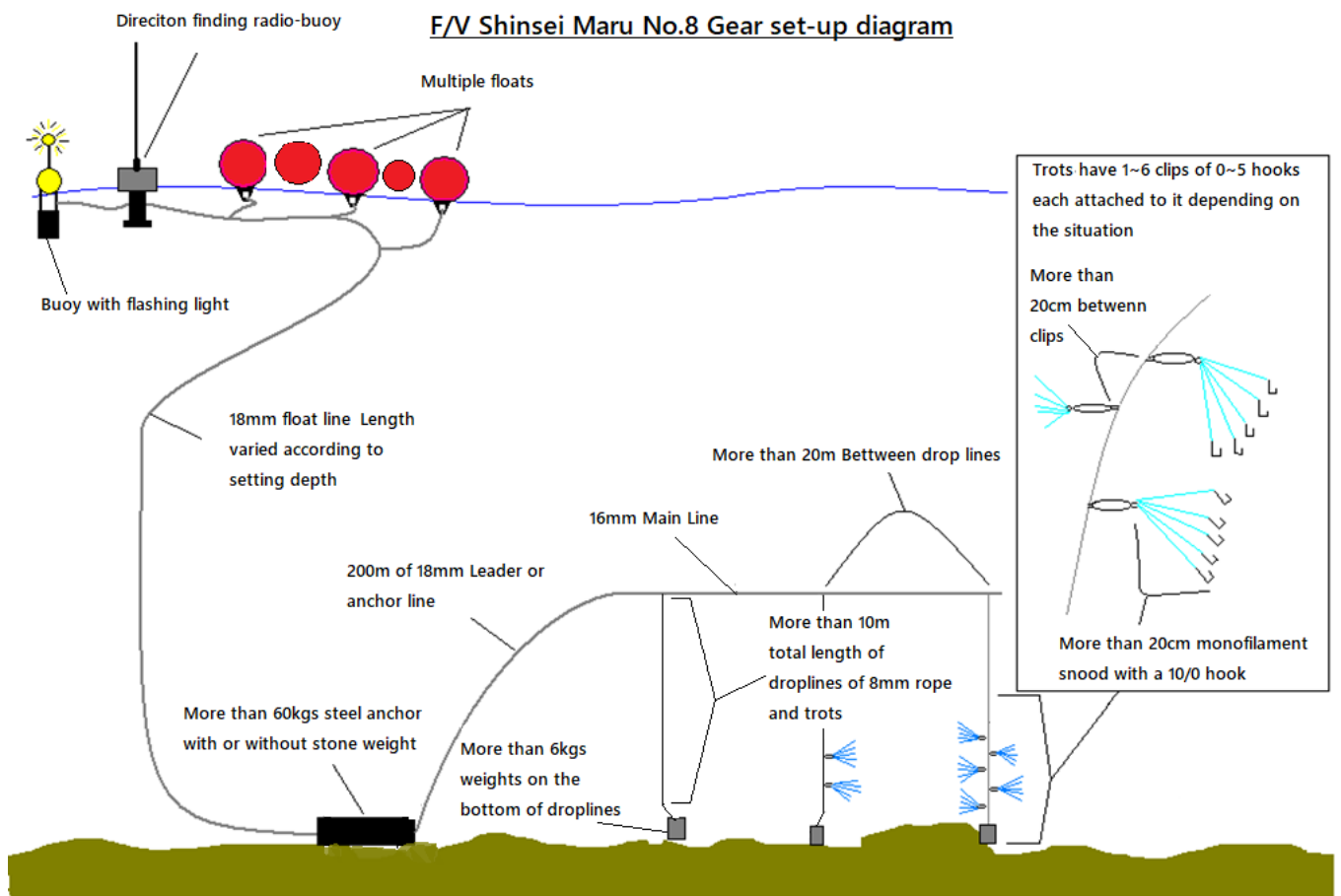
Fig.1 Configuration of Trot line
