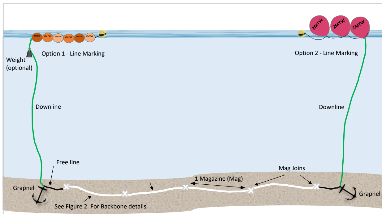
Figure 1: Typical Longline set up for the FV Janas
