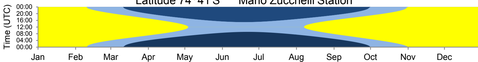
Latitude 74°41'S Mario Zucchelli Station
