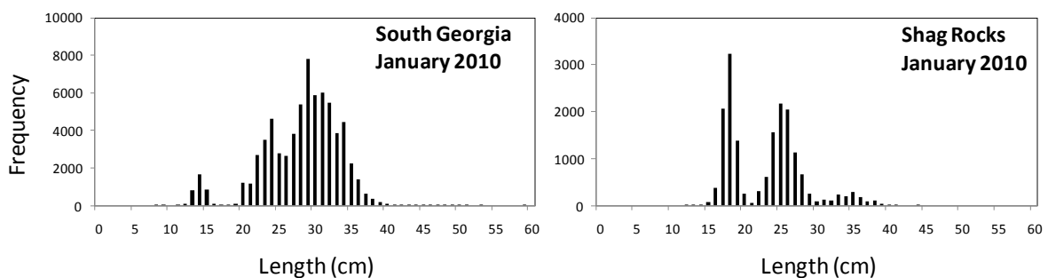
Figure 4: Catch-weighted length frequencies of Champtocephalus gunnari from the 2010 groundfish survey in Subarea 48.3.
