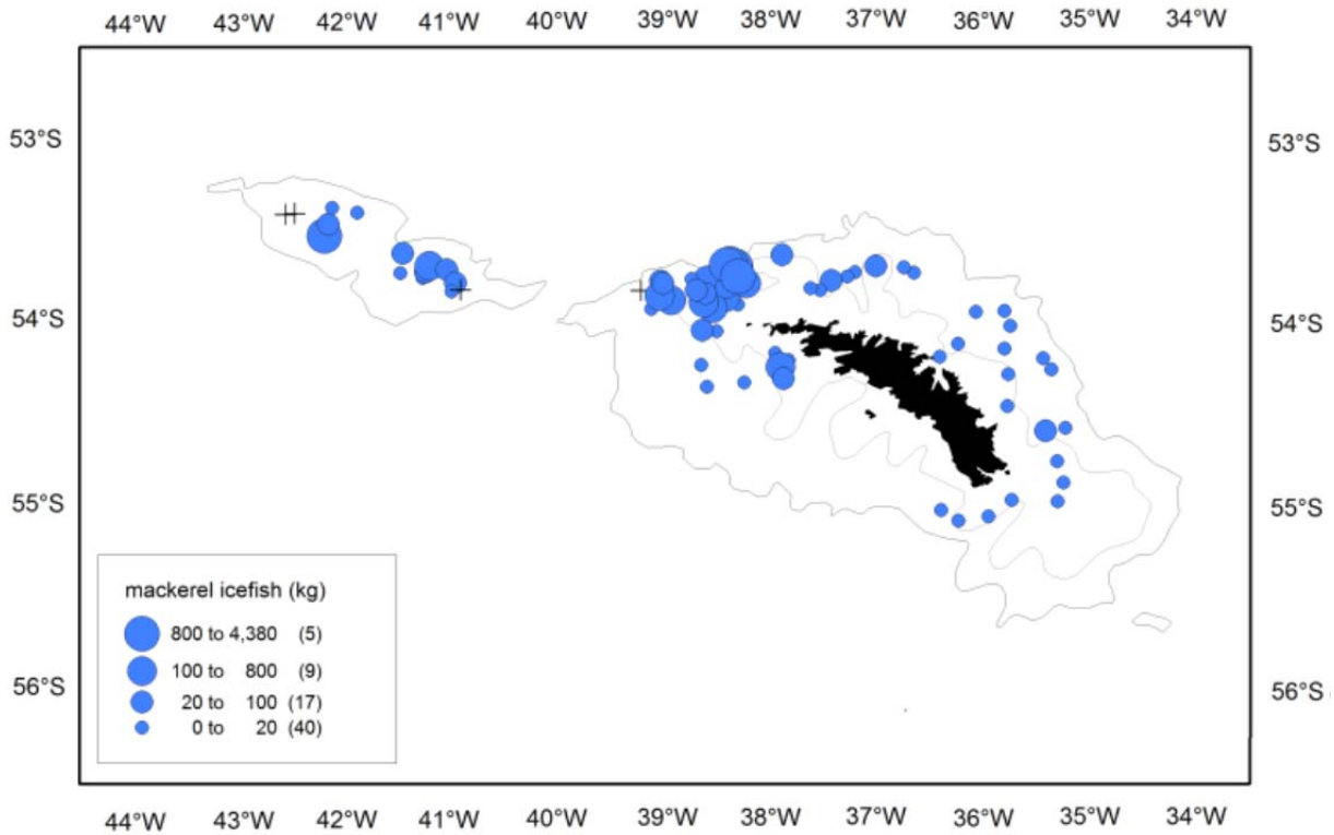
Figure 3: Champtocephalus gunnari catches from the survey in Subarea 48.3 in April 2010.
