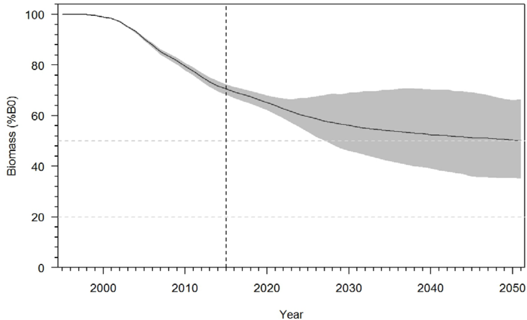
Figure A1.2: MCMC estimates of the spawning stock biomass trajectory as a percentage of initial biomass (black line) with the 90%ile (grey shading), projected out to 2051 for model R2. Dashed horizontal lines correspond to 50% B_0 and 20% B_0 .
