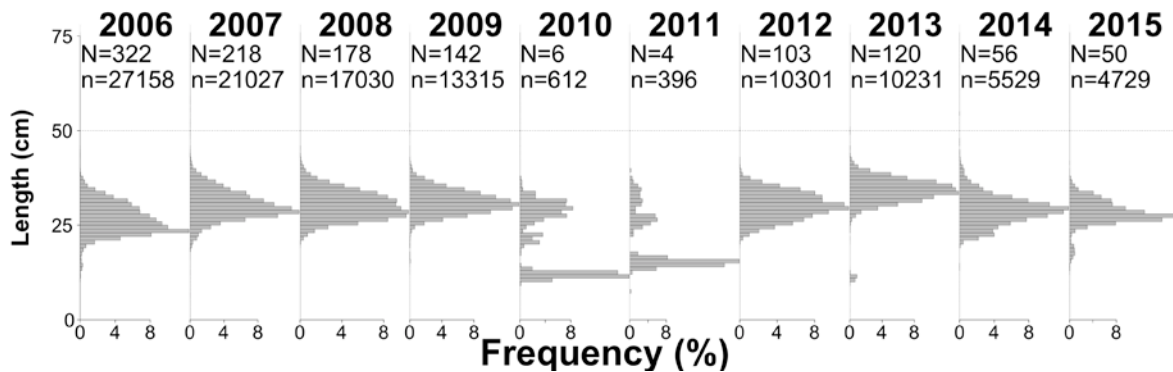
Figure 1: Length frequencies for Champsocephalus gunnari in Subarea 48.3 from observer data showing the number of hauls (N) and the number of fish measured (n) in each year at the top of each panel. Note that in 2010 and 2011 data are primarily from research hauls.
